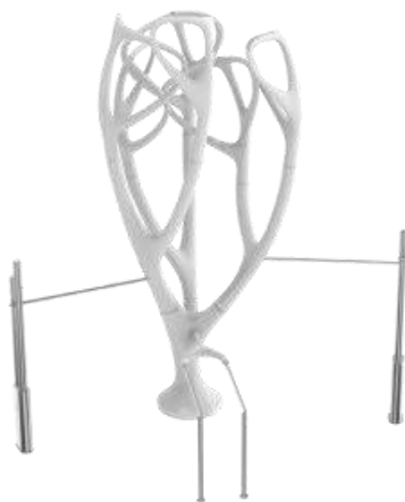
Unparalleled Tree
