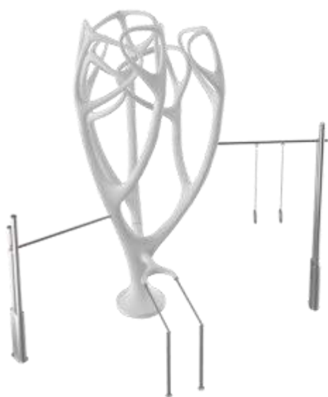
Full Tree
